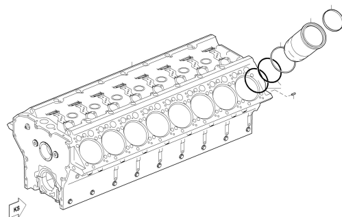
CRANKCASE UPC.06A01 1916
